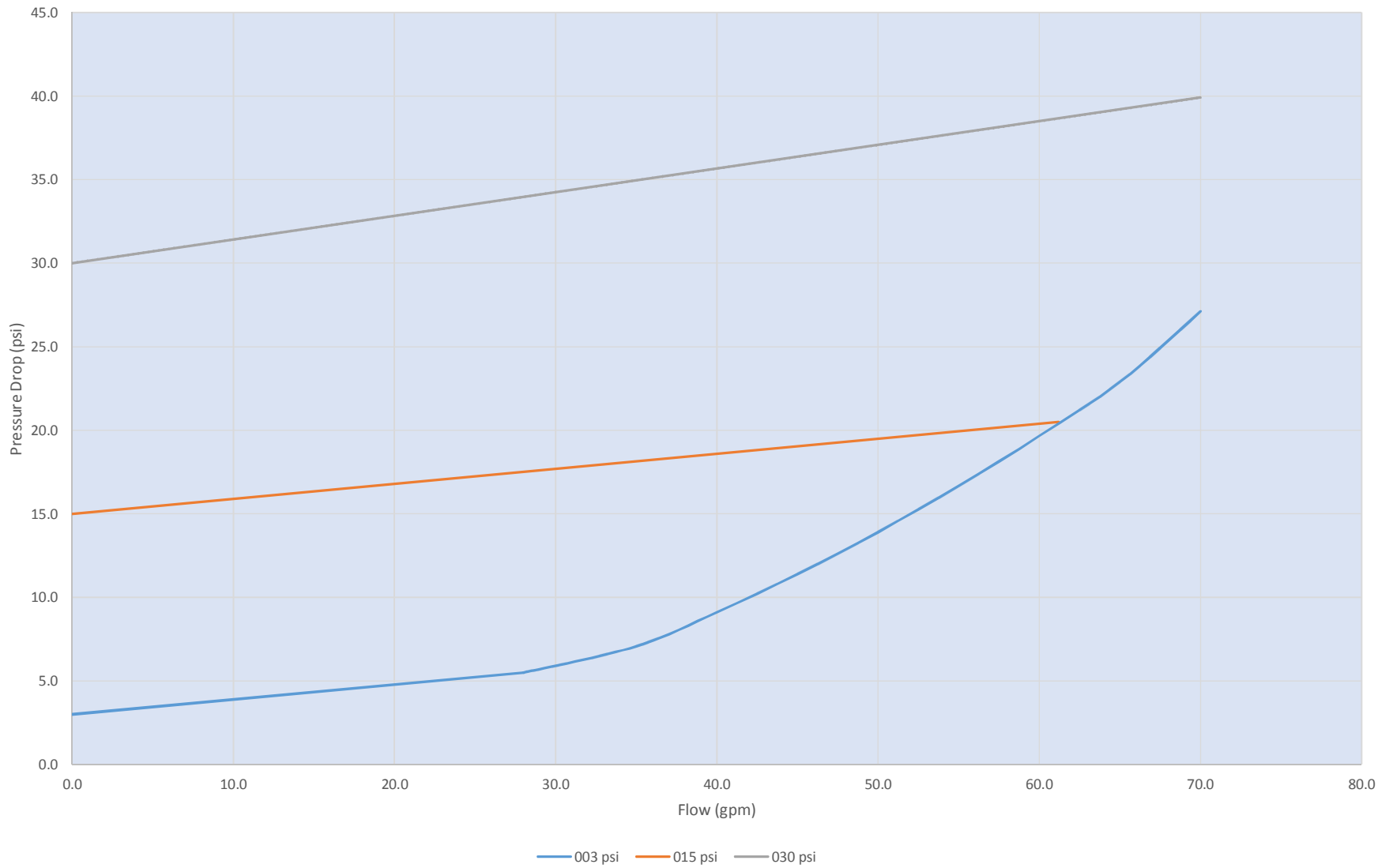
ICT-B-20 Pressure Drop versus Flow (ISO 68 Oil, T=100F )
