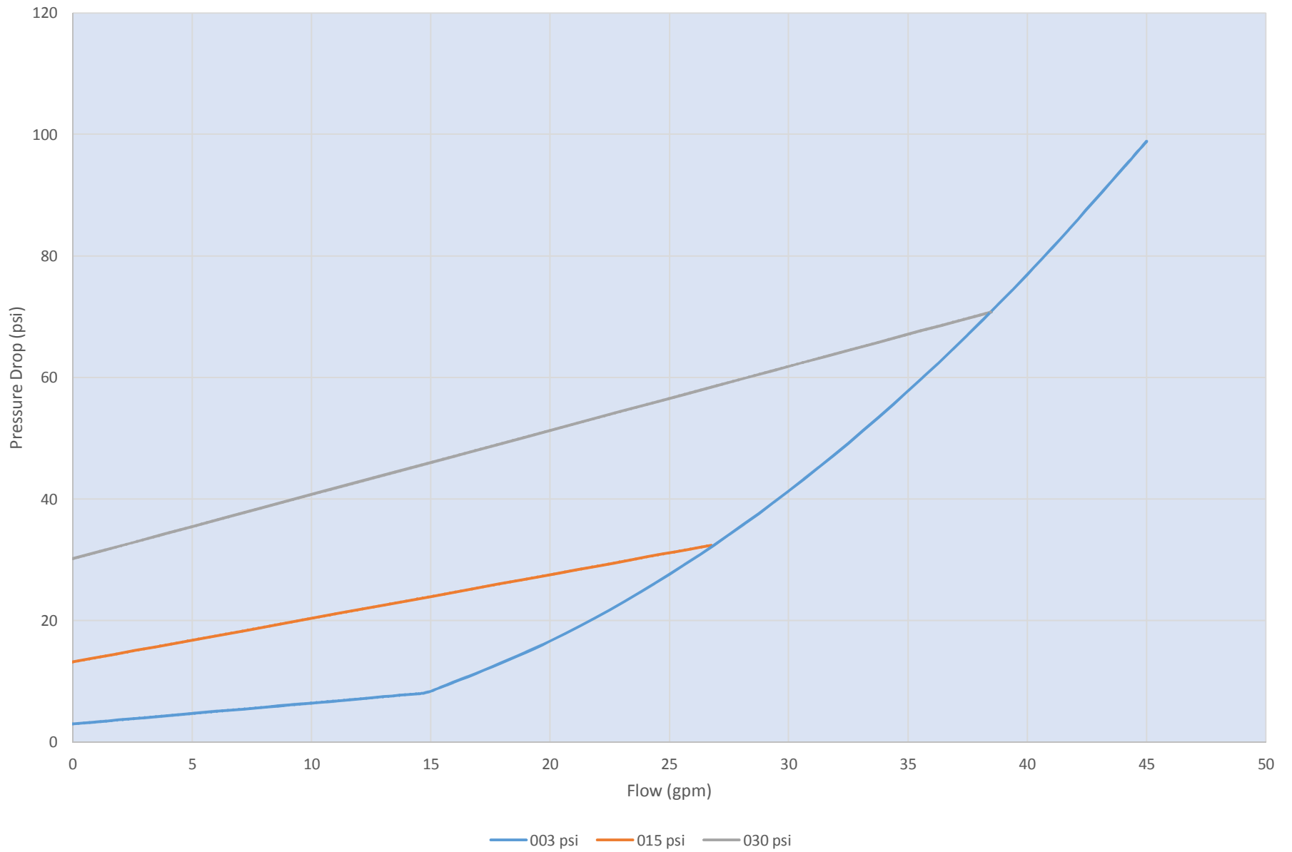
ICS-C-16 Pressure Drop versus Flow (ISO 68 Oil, T=100F )
