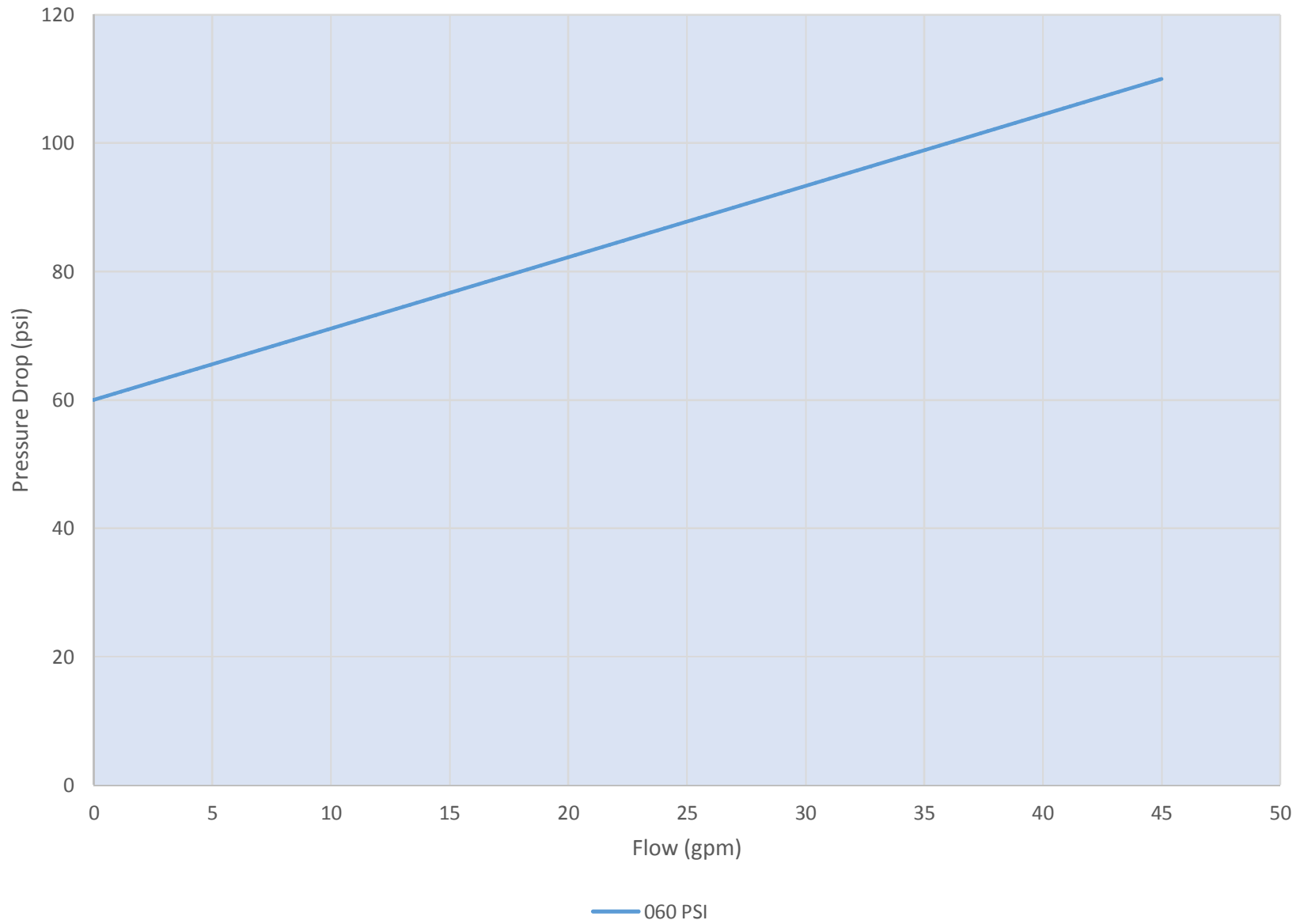
ICS-C-16 Pressure Drop versus Flow (ISO 68 Oil, T=100F )
