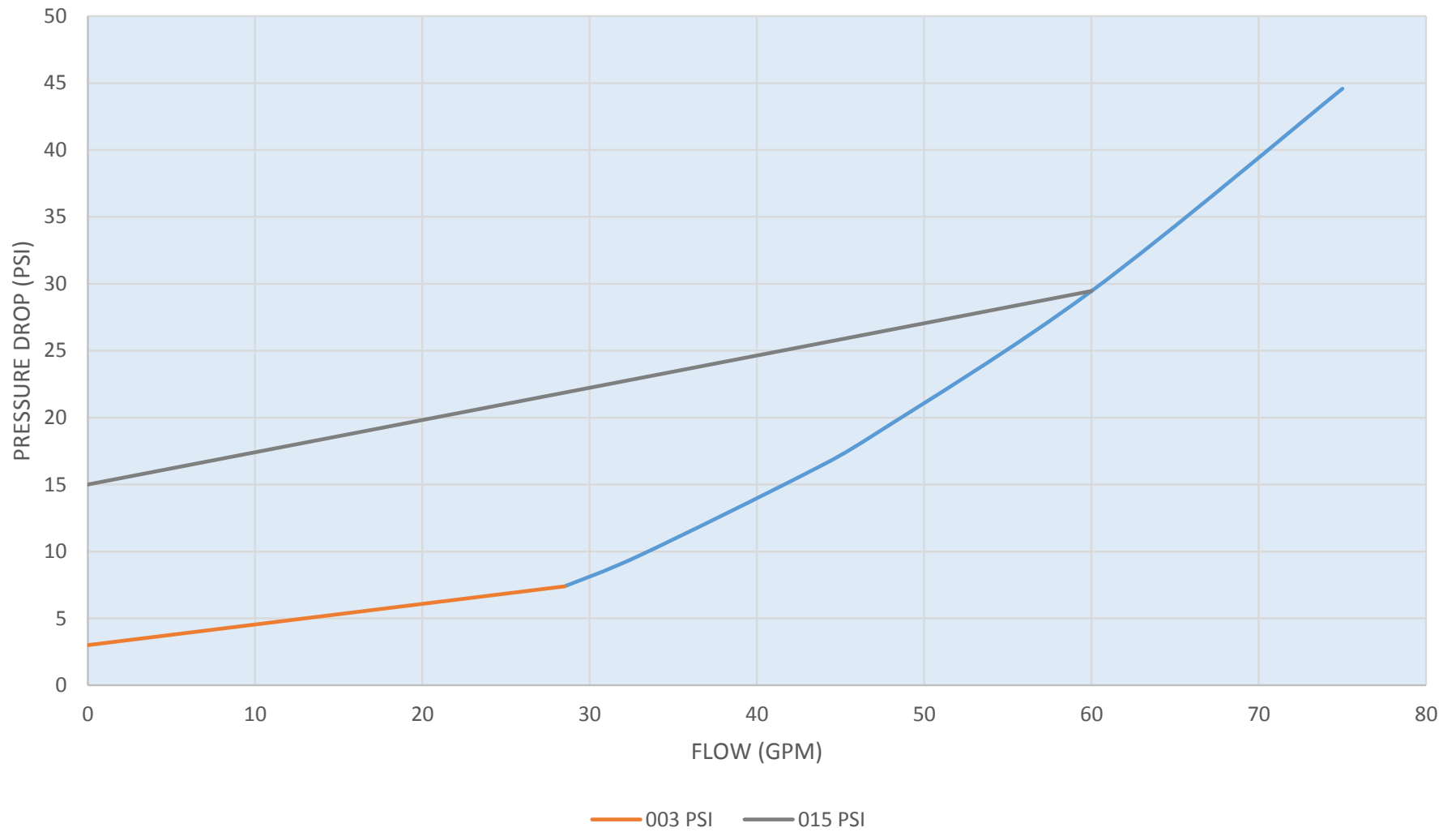
IGS-A-20 FLOW VERSUS PRESSURE DROP SIDE PORTED FLOW (INLET-AXIAL, OUTLET-RADIAL) ISO 68 OIL, 100F
