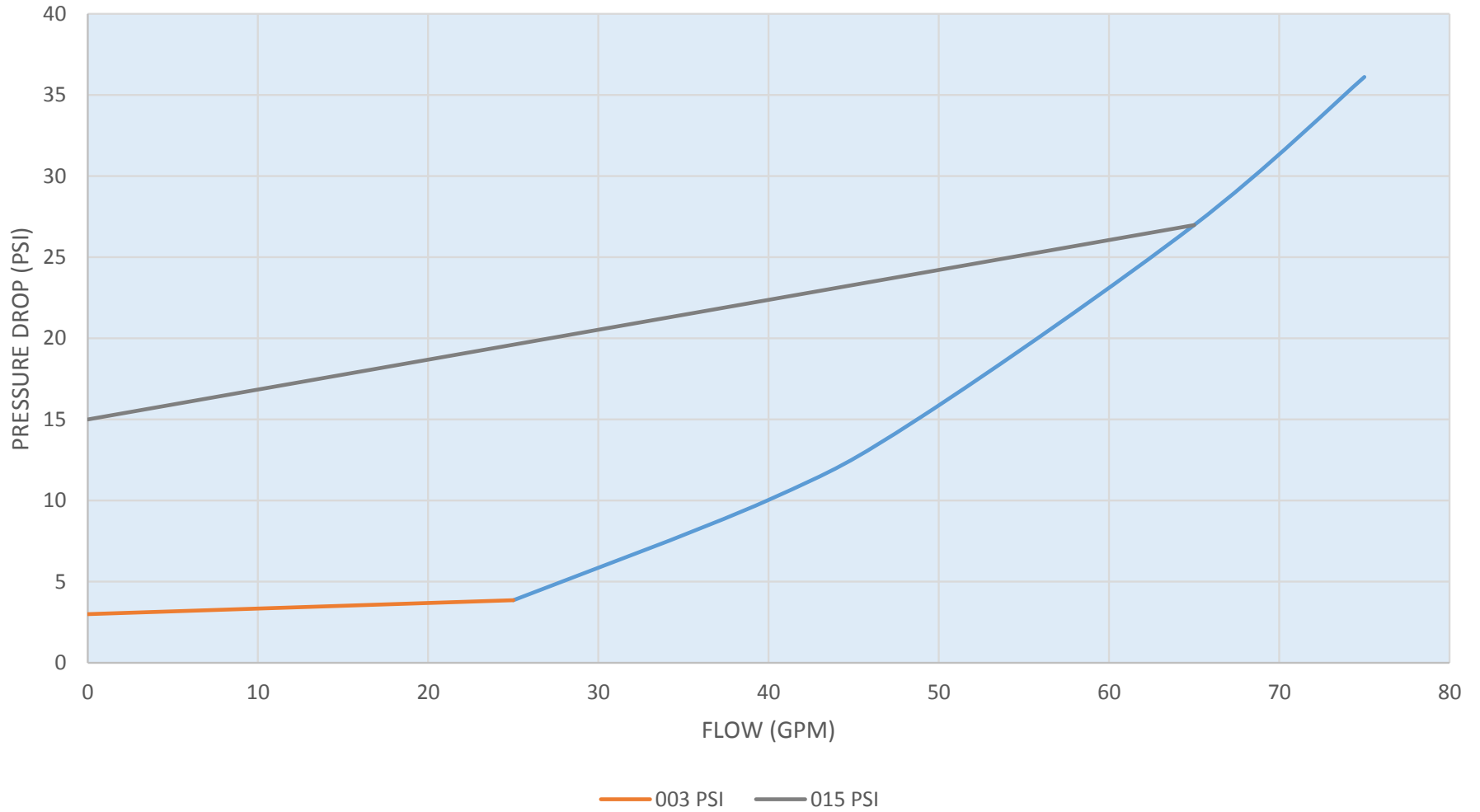
IGS-A-20 FLOW VERSUS PRESSURE DROP SIDE PORTED FLOW (INLET-AXIAL, OUTLET-RADIAL) 1.968" DIA x 1.00" ANNULAR CAVITY UNDERCUT ISO 68 OIL, 100F
