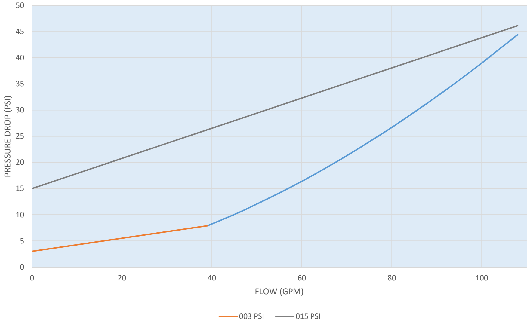
IGS-A-24 FLOW VERSUS PRESSURE DROP SIDE PORTED FLOW (INLET-AXIAL, OUTLET-RADIAL) ISO 68 OIL, 100F
