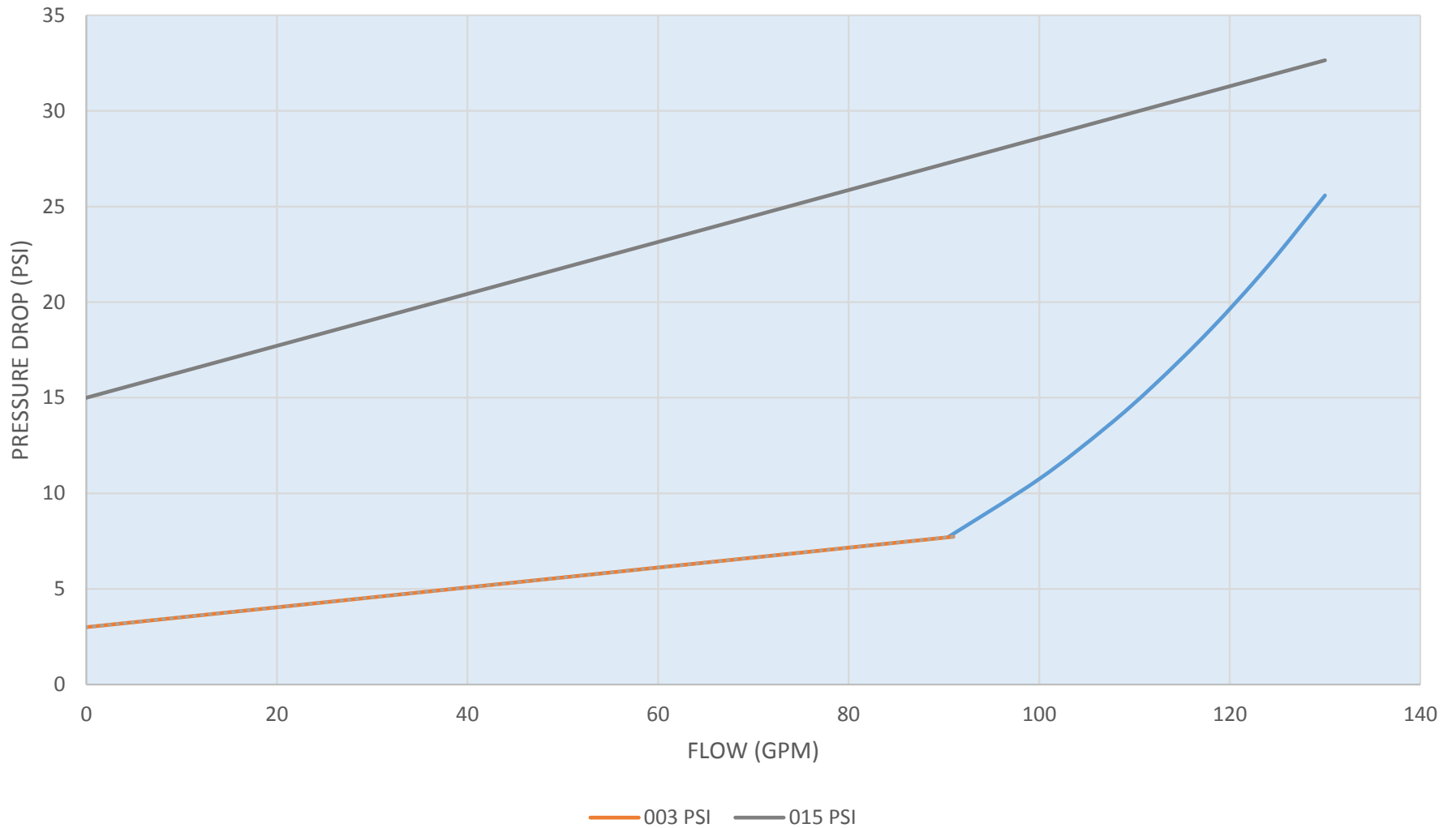
IGS-A-32 FLOW VERSUS PRESSURE DROP SIDE PORTED FLOW (INLET-AXIAL, OUTLET-RADIAL) ISO 68 OIL, 100F
