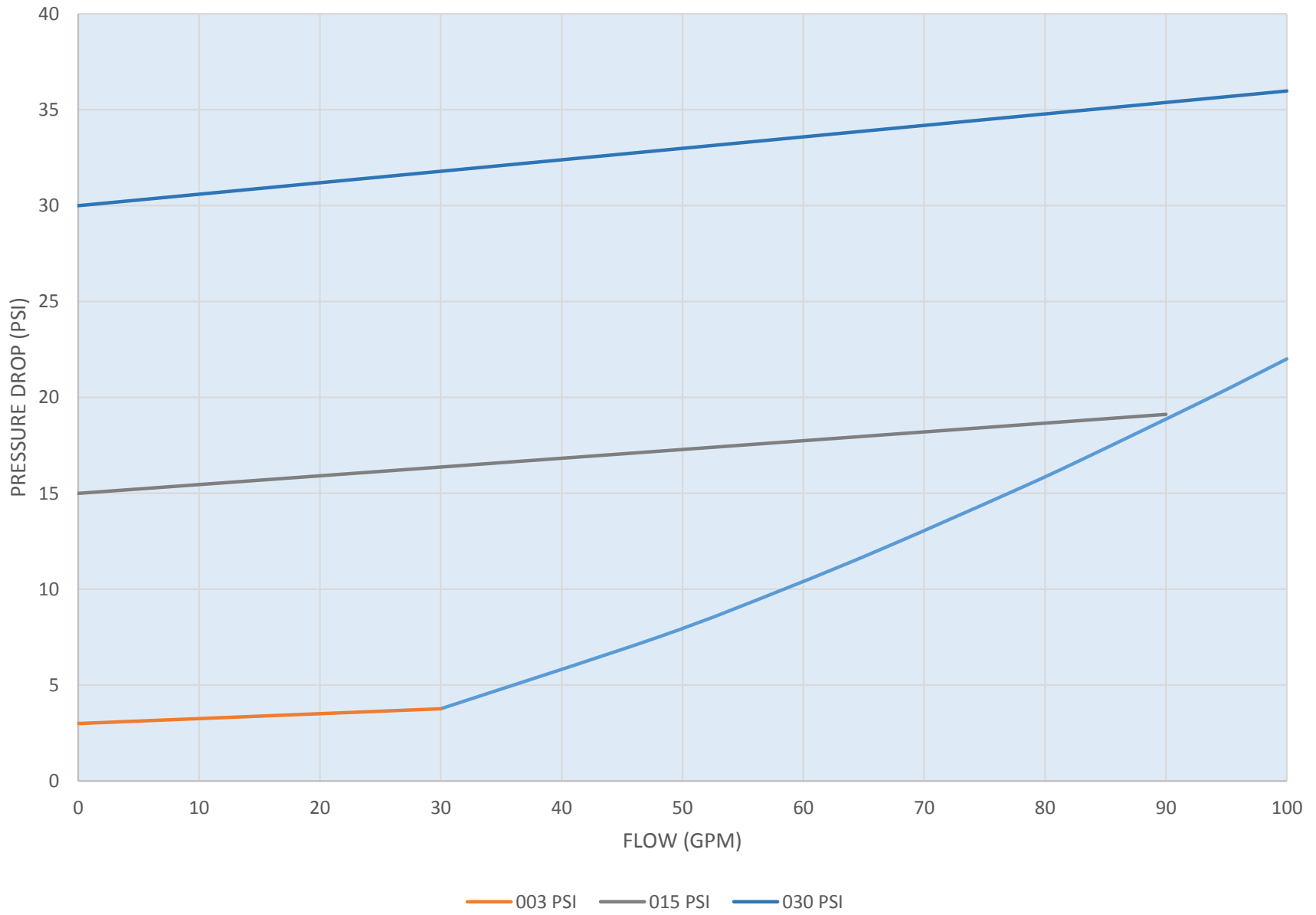
ICT-B-24 FLOW VERSUS PRESSURE DROP ISO 68 OIL, 100F
