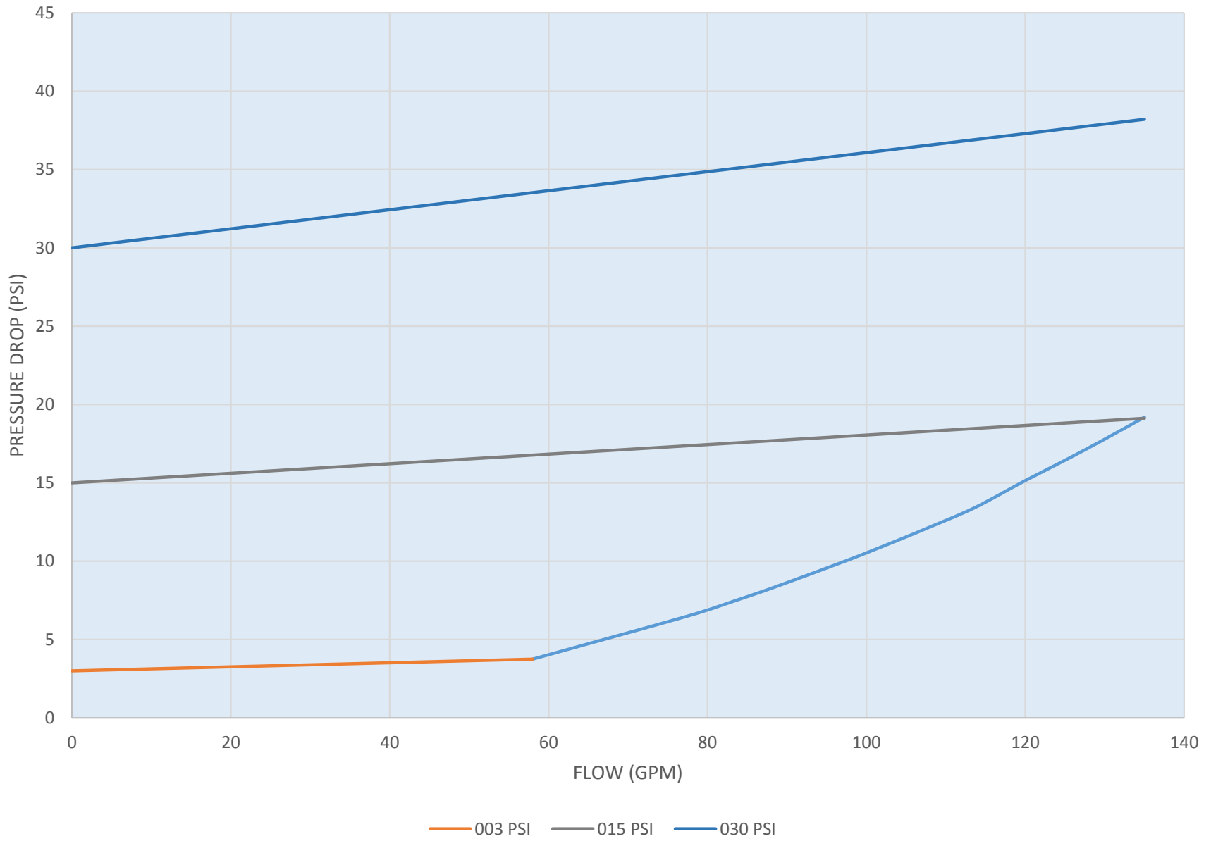
ICT-B-32 FLOW VERSUS PRESSURE DROP ISO 68 OIL, 100F
