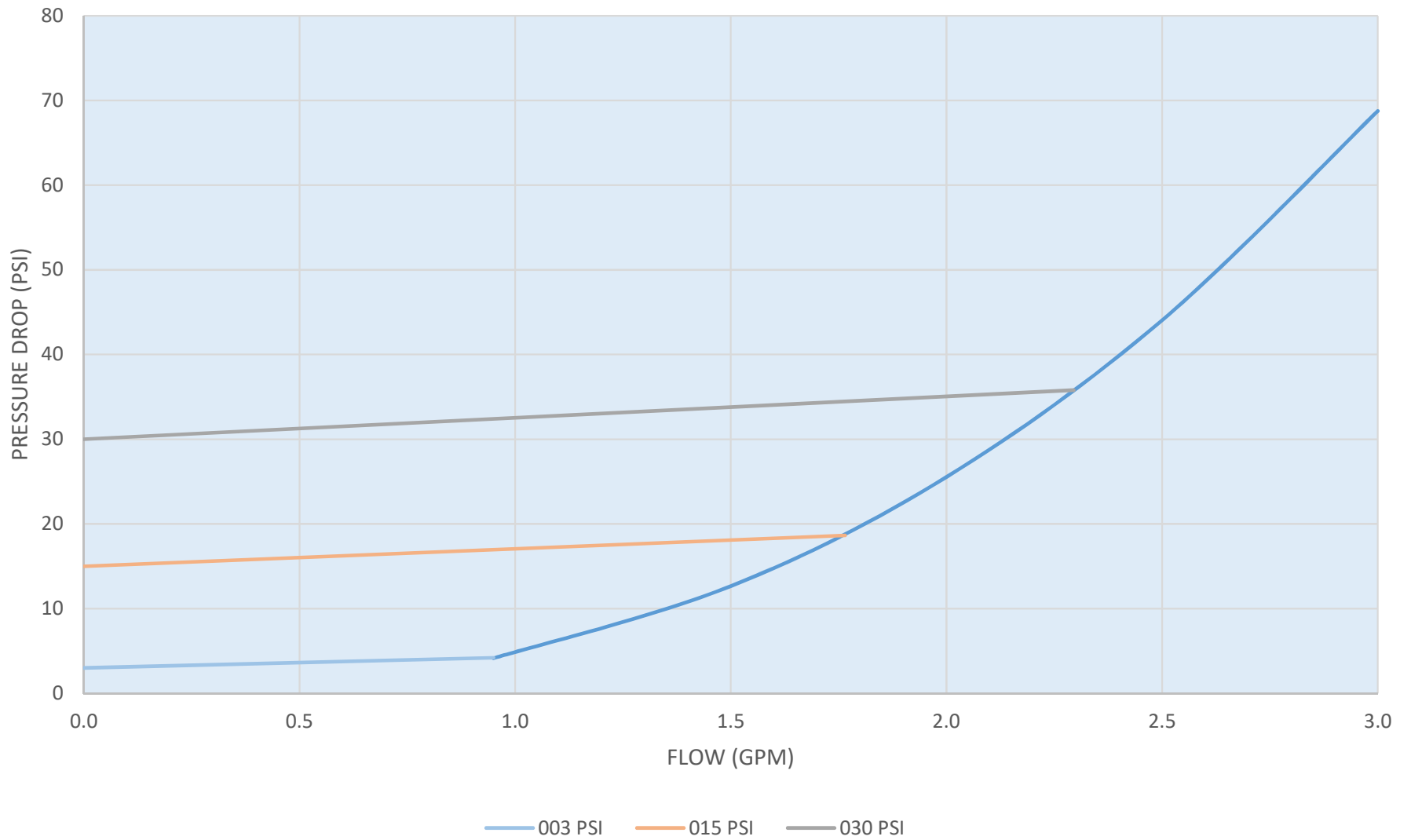
ICT-B-04 FLOW VERSUS PRESSURE DROP ISO 68 OIL, 100F
