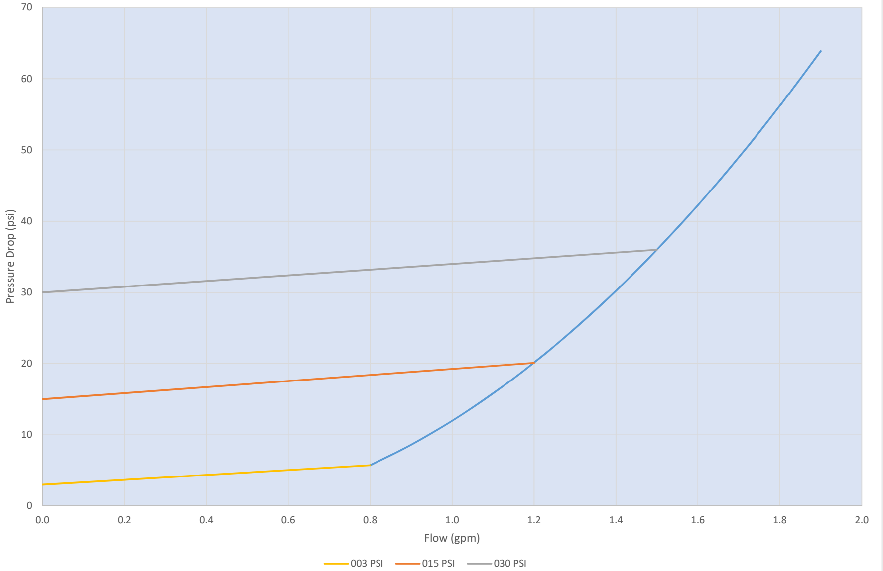
ICT-B-03 Pressure Drop versus Flow (ISO 68 Oil, T=100F )
